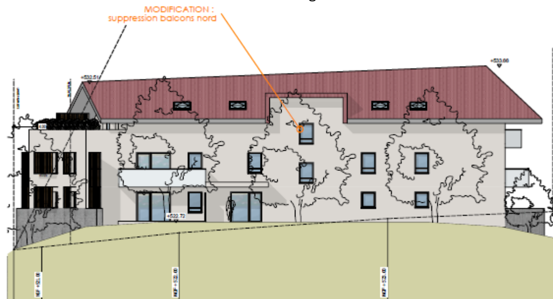
BATIMENT I - FACADE NORD
