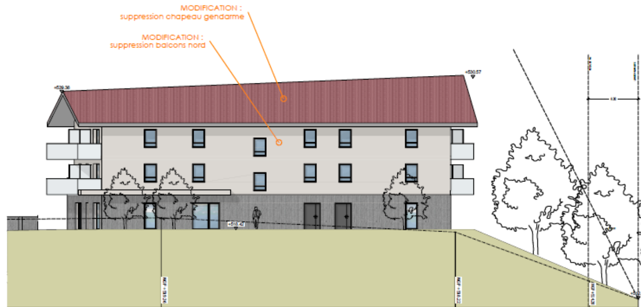
BATIMENT H - FACADE NORD
